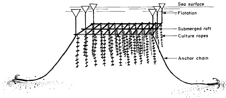
Fig. 8. Scheme of a submersible raft for mussel culture (drawn after Nayar et al. 1980).
