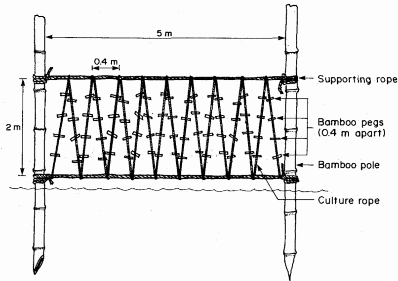
Fig. 7. "Rope-web" method for the culture of Perna viridis employed in the Philippines (after Yap et al. 1979, modified).
