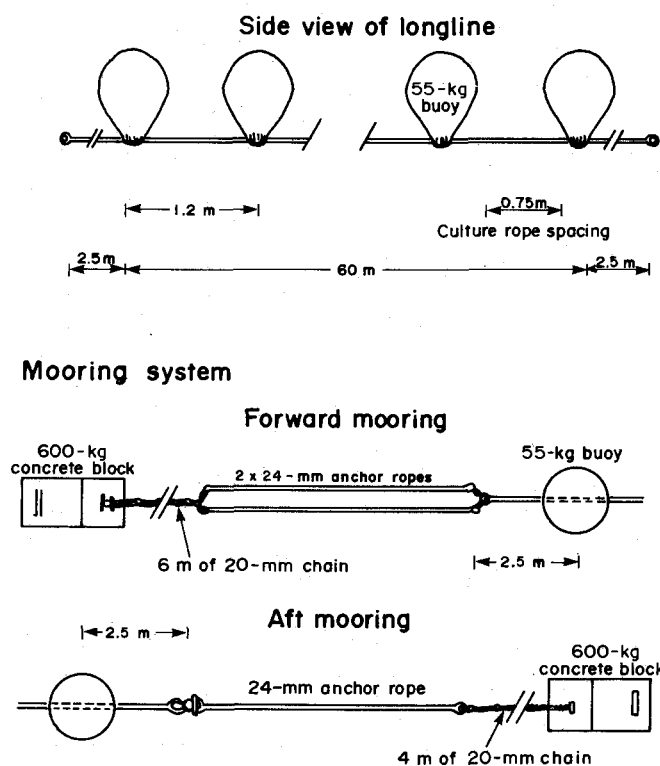
Fig. 10. Construction details for a standard 60-m longline system: reproduced Johns and Hickman (1985) with kind permission from the New Zealand Fisheries Research Division.
