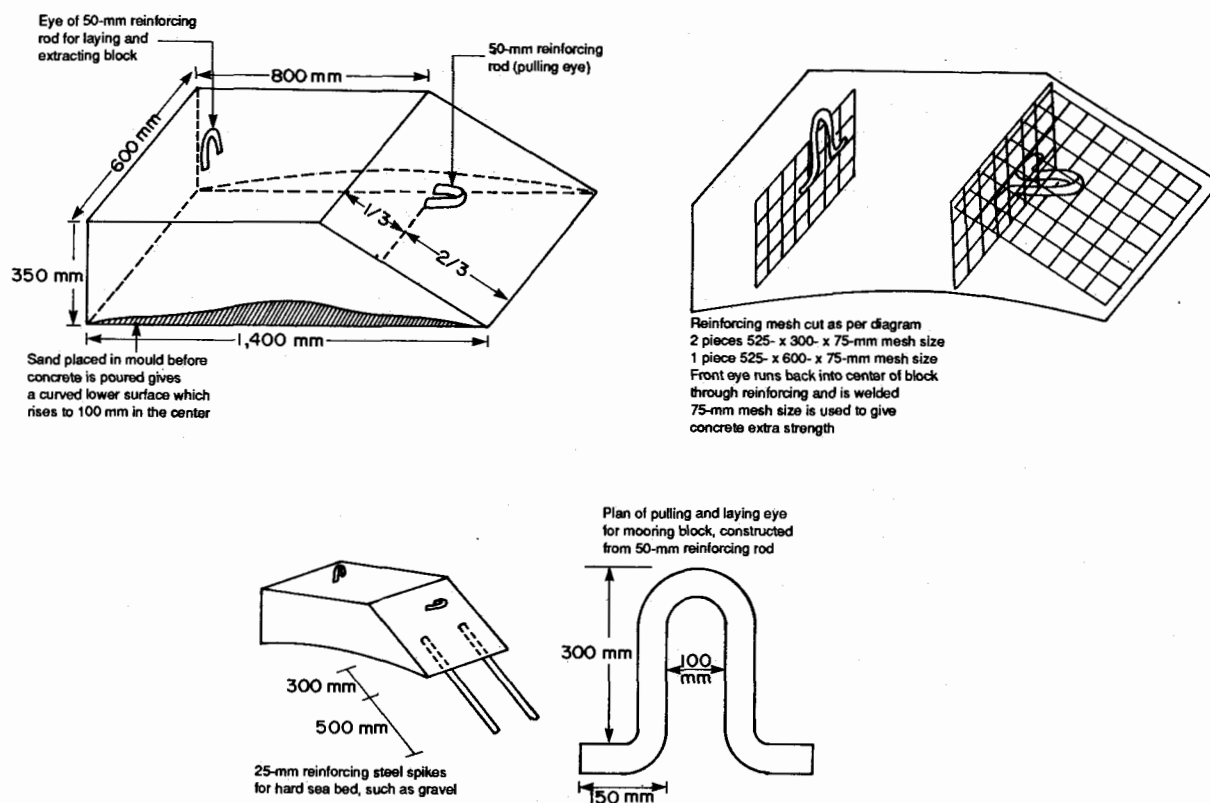
Fig. 9. Construction details for a 500-kg mooring block: reproduced Johns and Hickman (1985) with kind permission from the New Zealand Fisheries Research Division.
